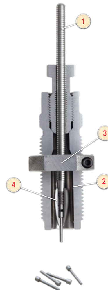
The replaceable decap pin (No. 390222) is unique to Hornady® Dies.
